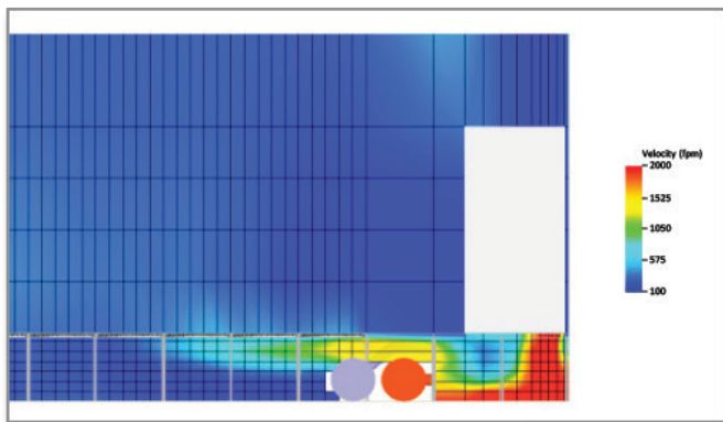
Picture: CFD analysis of same layout with different calculation grids
