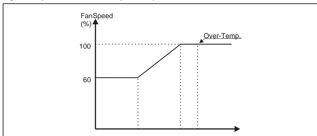
Figure 4: Hysteresis line for fan speed/temperature
