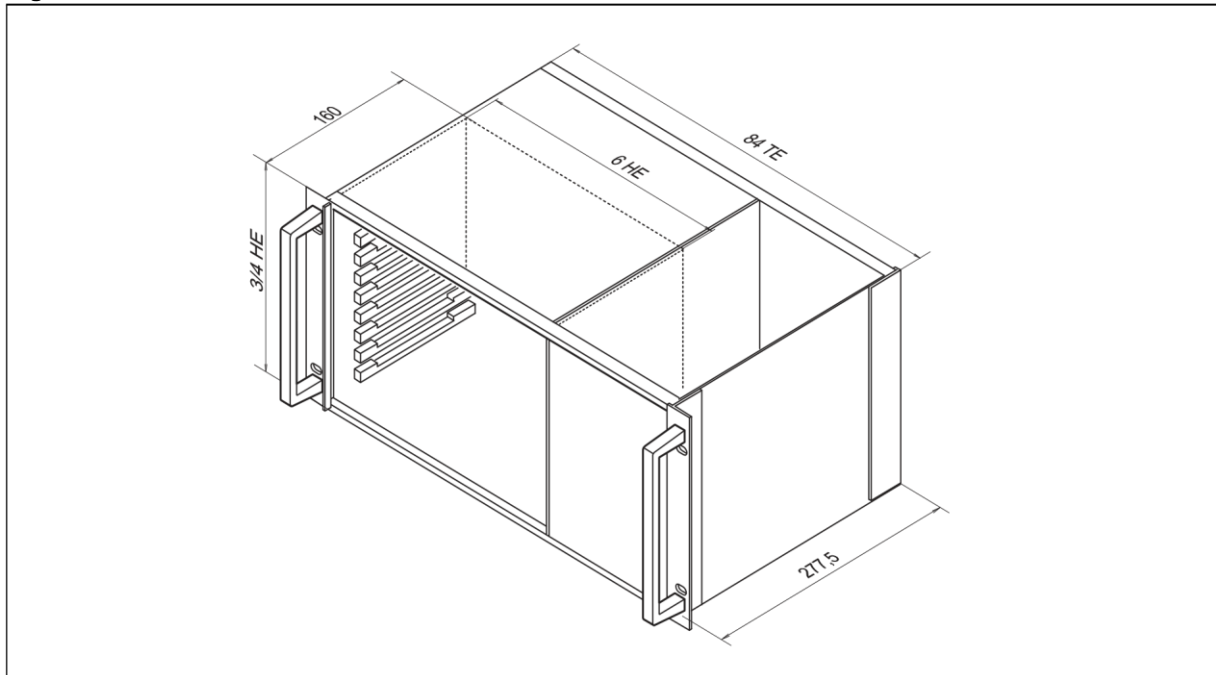
Figure 7: Dimensions
