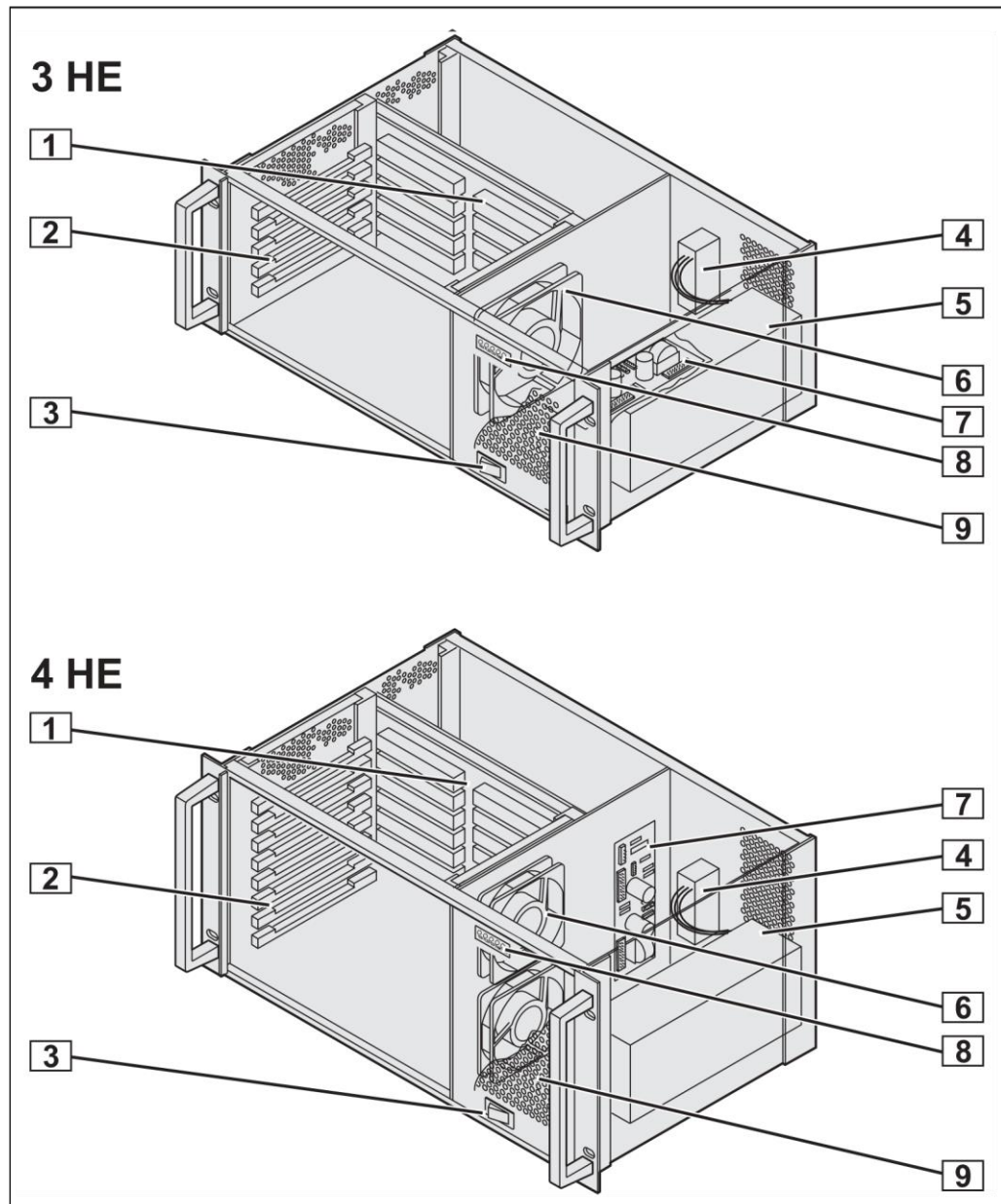
Figure 1: Subrack Systems Overview
