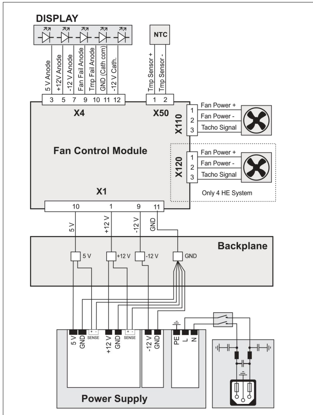
Figure 2: Wiring Diagram
