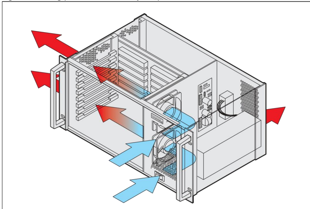
Figure 3: Cooling (illustrated on a 4 U system)
