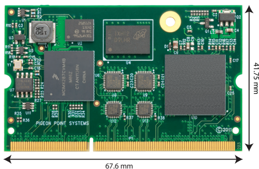
Mezzanine Module for ATCA (ShMM-700R) and VPX Chassis (ChMM-700R)
