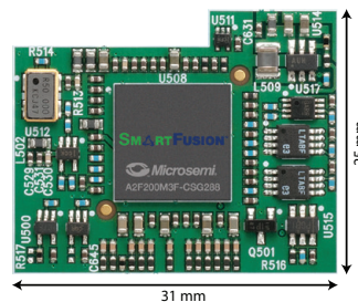
Reference IPMC for ATCA or VPX
