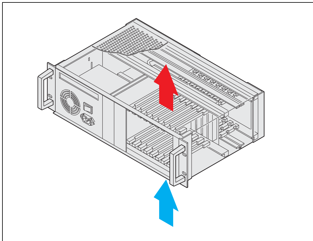
Figure 2: Airflow
