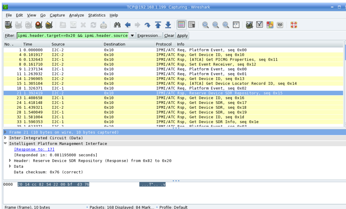
Figure 16: Filtered trace
