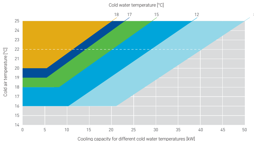
Graph of cold air temperature against cooling capacity for in-row heat exchanger
