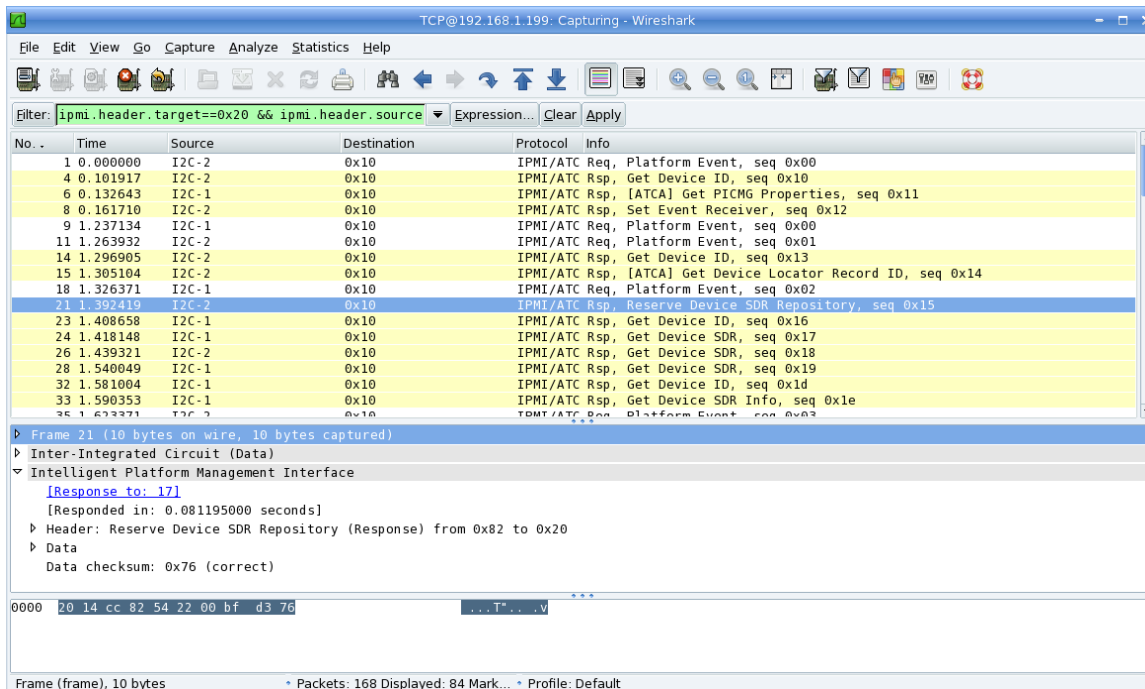
Figure 16: Filtered trace
